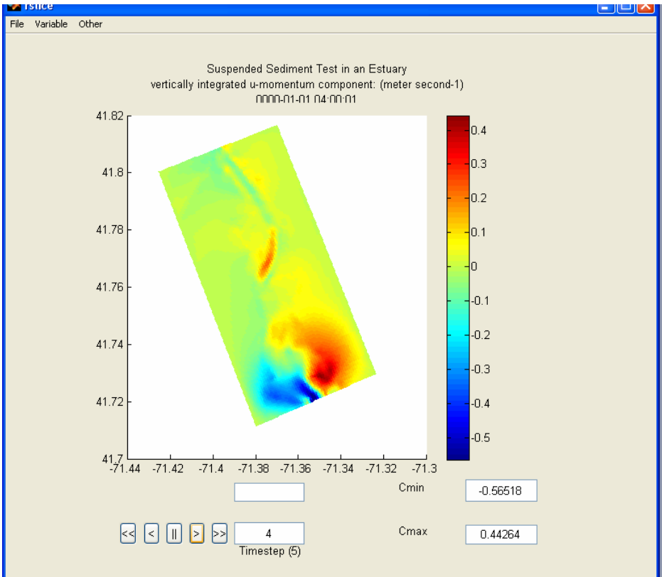
Figure 3 Simulated currents
